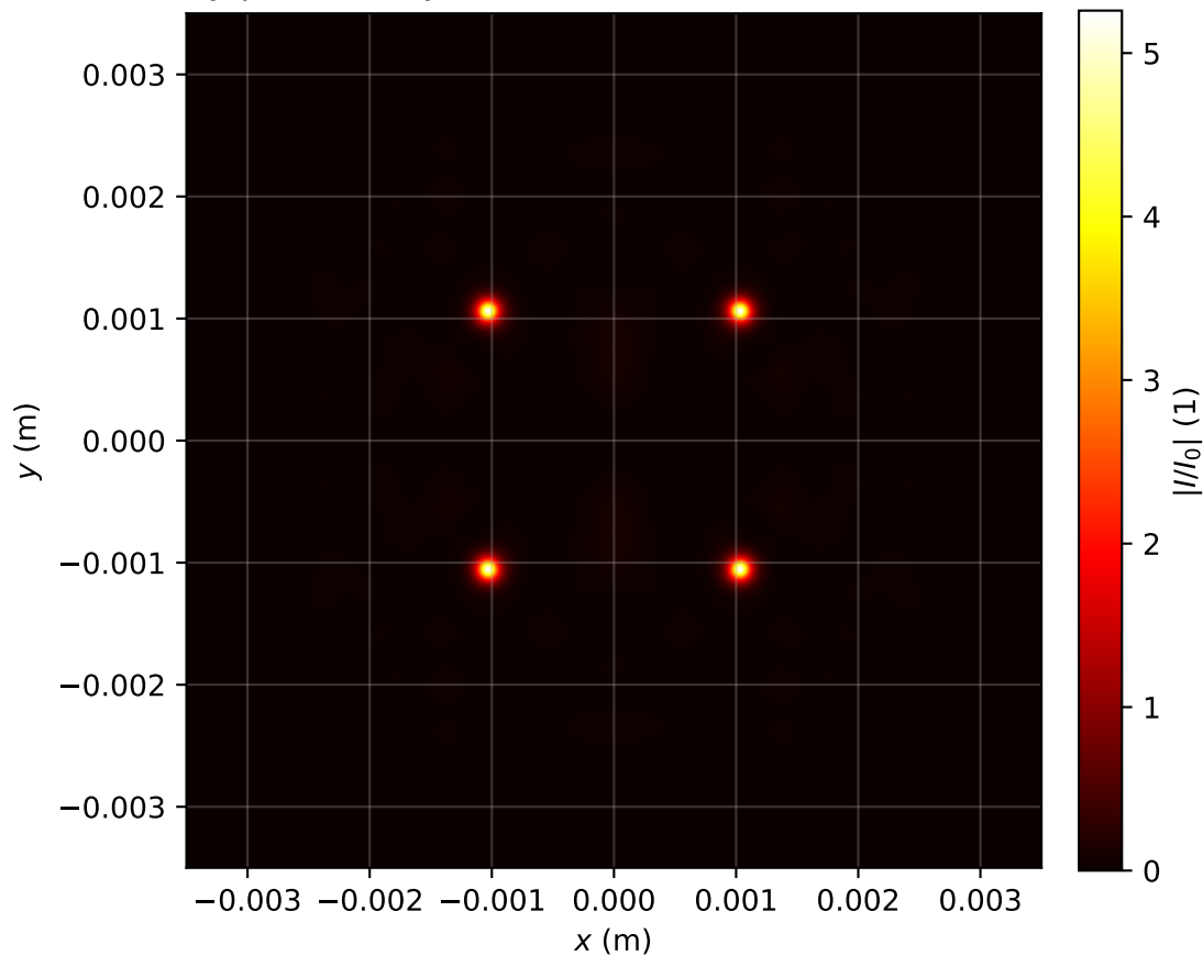
Intensity profile I(x, y, z = 3.901)/I_0 , P_{in}=9.0P_{cr} , artificial time
